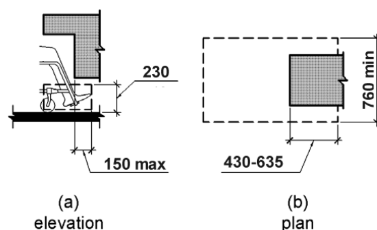
Figure 4: Toe clearance
