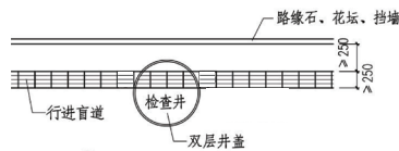
② 盲道遇检查井平面布置
